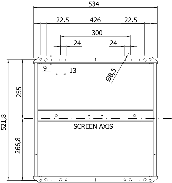
WALL FIXING POINTS
