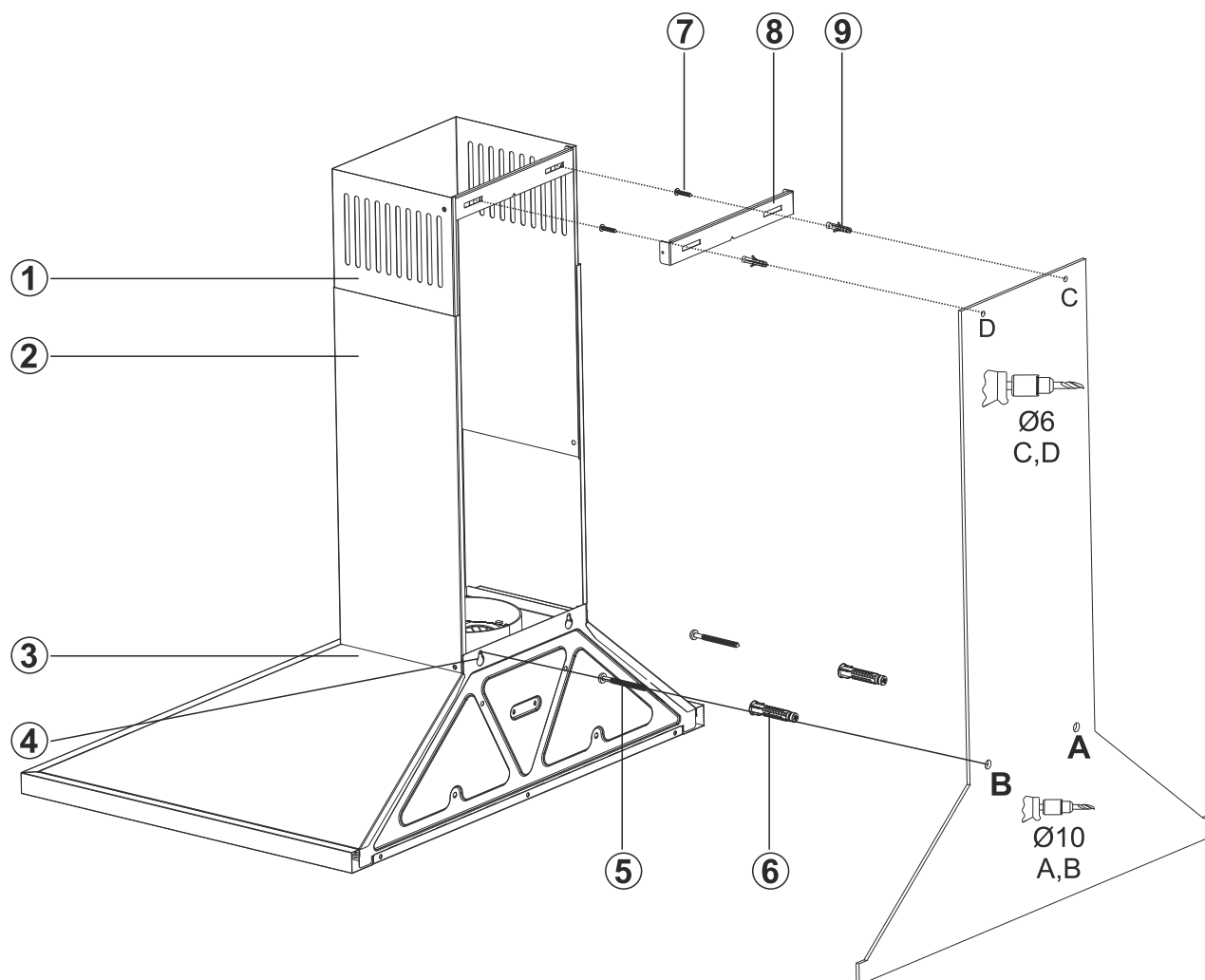
Fig. 12: INSTALLATION AND PARTS
