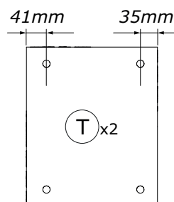
TR02684 325x268x16mm
