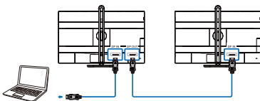
Multi-stream transport
